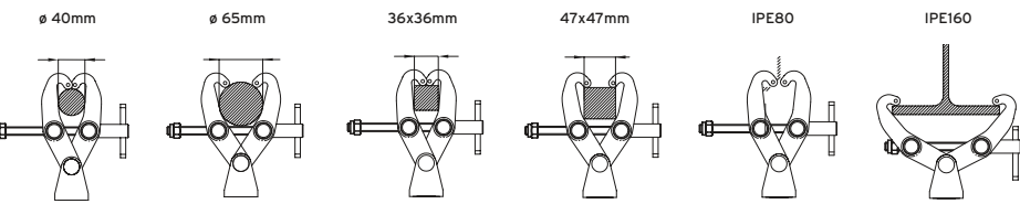
Clamp Range: 40mm to 65mm Clamp Range: 36mm to 47mm Clamp Range: IPE 80 to IPE 160 HEB 80 to HEB 160
