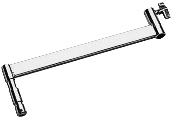
F100 JUNIOR OFFSET ARM 28MM PIN / 28MM SOCKET 1,5kg 3.3lb 28mm 1" 1/8" 28mm 1" 1/8" Length: 50cm (19.7").
